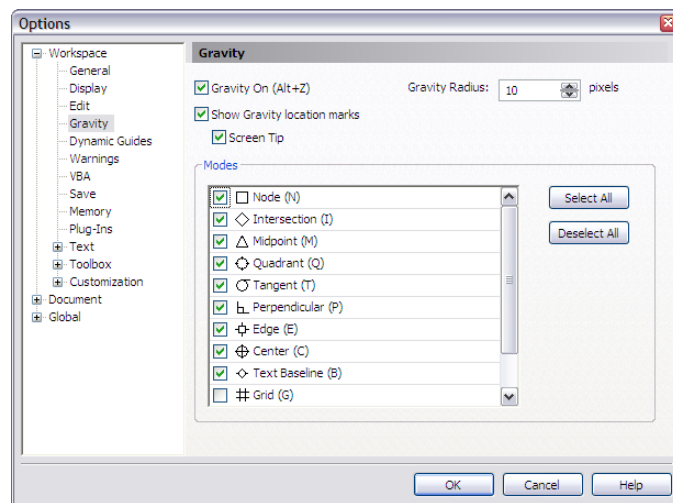
Users can customize the behavior of gravity snapping.
